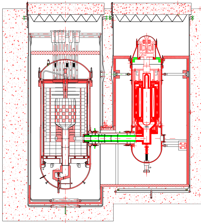
Figure A-3. HTR-10 cross-section.
